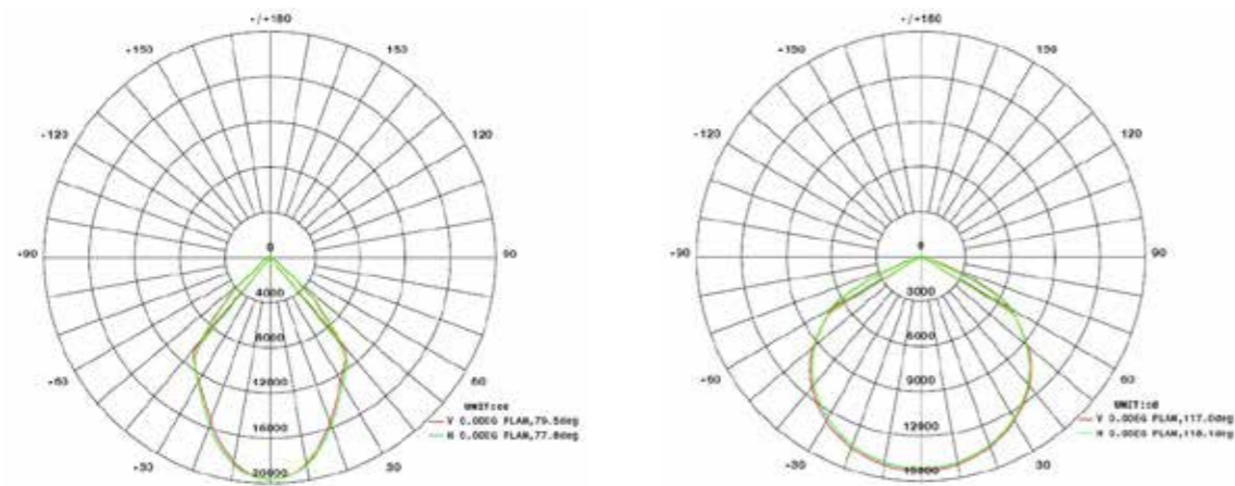
Light distribution curve
